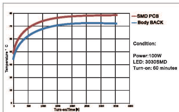
Temperature Rise
