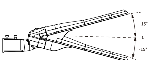
Horizontal Installation ±0-5-10-15°
